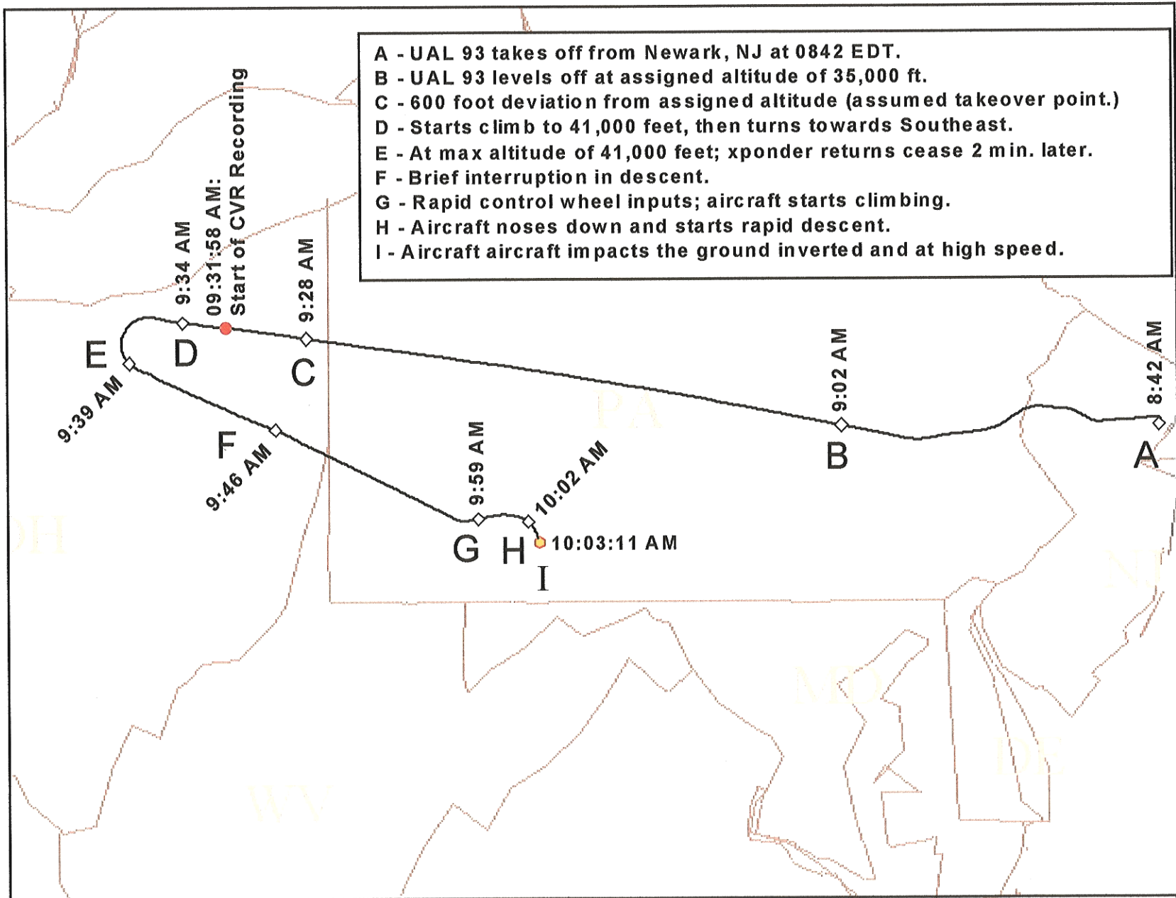
Figure 1. UA-93 Radar Ground Track
